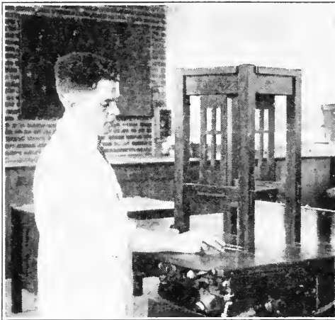
FIG. 422. SCRIBING LEGS TO LENGTH.
